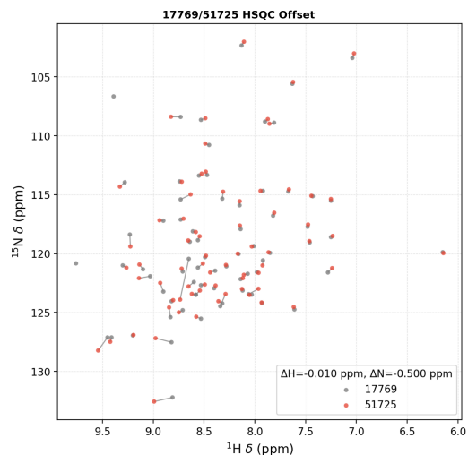
SI Fig. S25E. Apo vs apo control study for BMRB 17769 and 51725. This case involves ubiquitin. There is a sequence mismatch at position 12 (T12C; wild-type Thr in BMRB 17769, Cys in BMRB 51725). 81.2% of the CSPs for this control are below 0.05 ppm.
